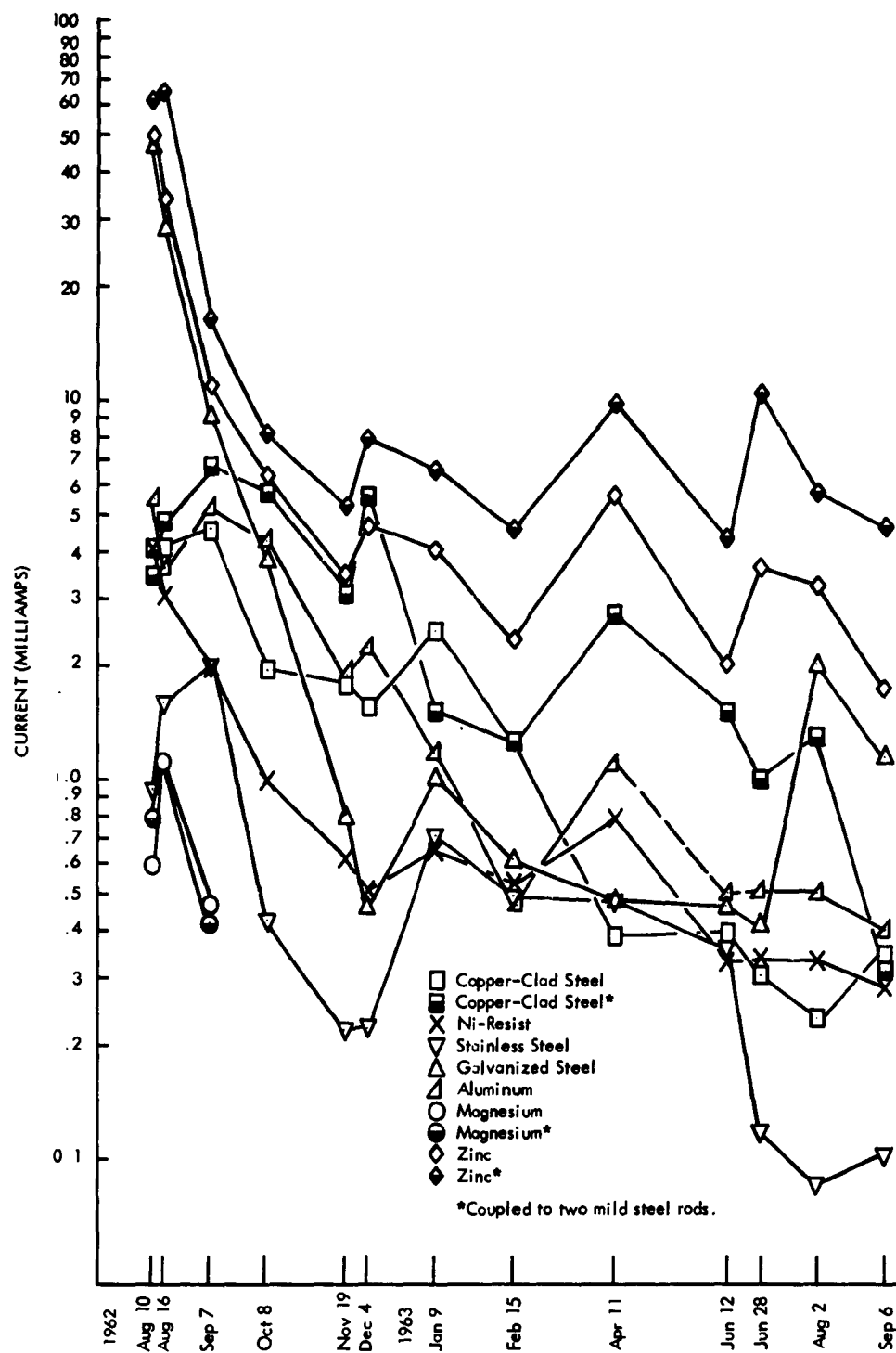
Figure 9-B. Current Flow in Couples. Mugu Site
