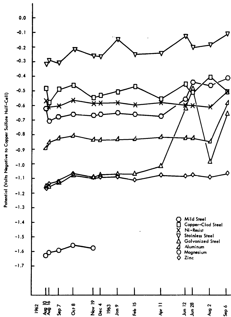
Figure 7-B. Potential of Single Rods. Mugu Site
