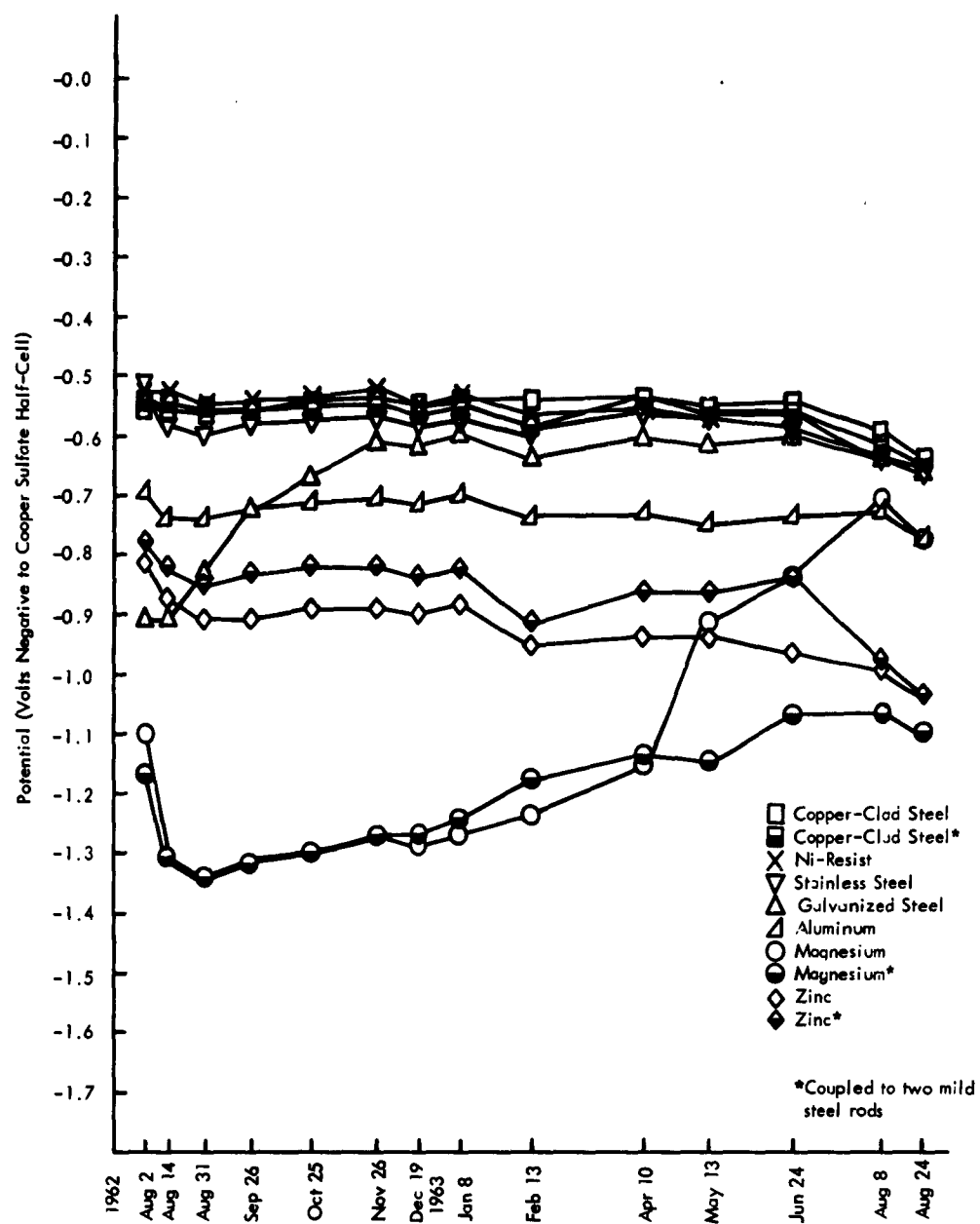
Figure 3-B. Potential of Coupled Rods. NCEL Site - 1 Year Group.
