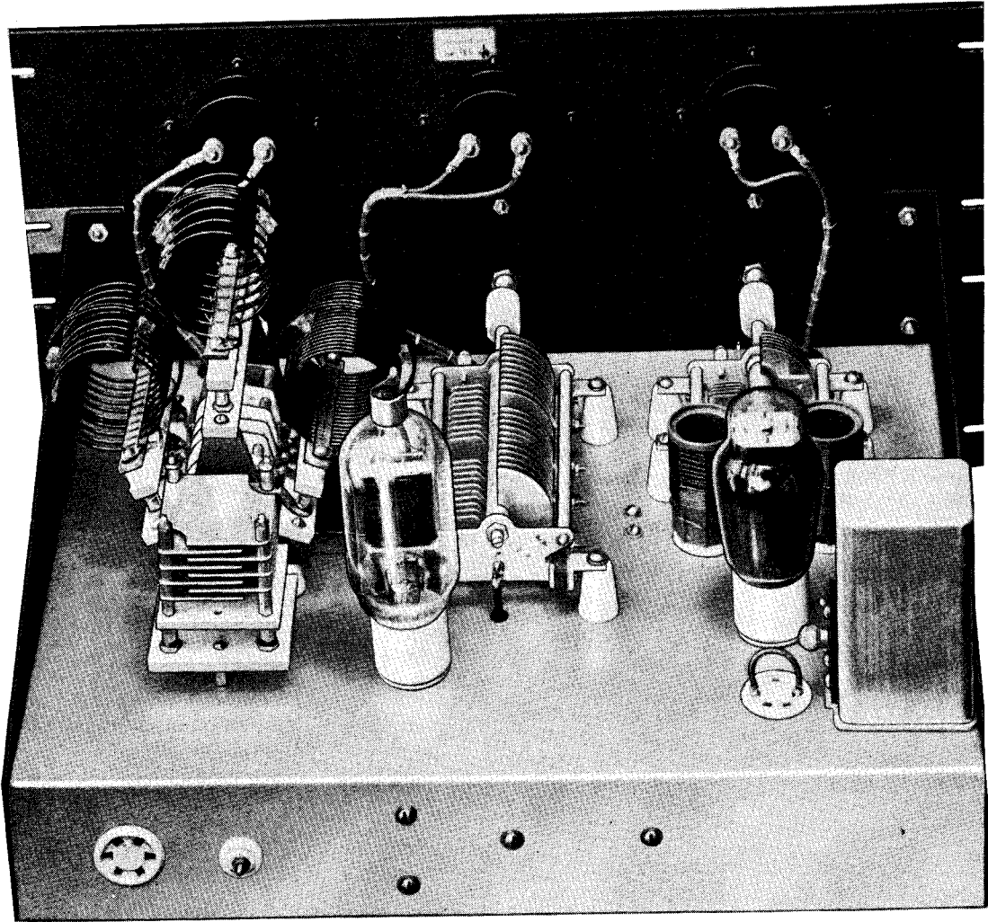
Top View—QBC Unit No. 1
