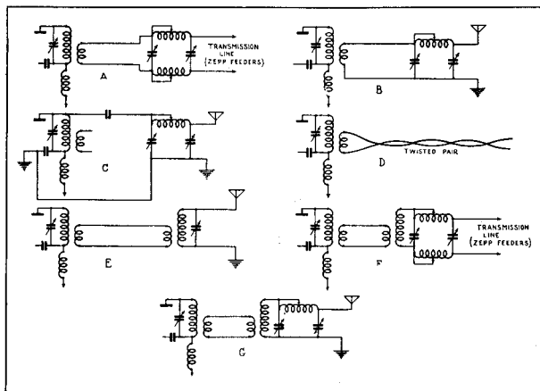
ANTENNA CHART
