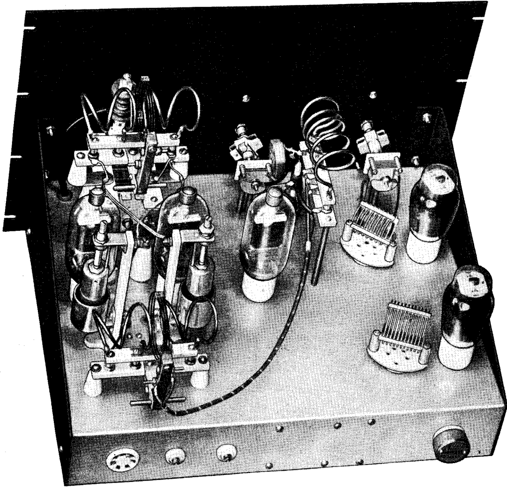
Top View—Unit No. 2—High Freq. R.F.
