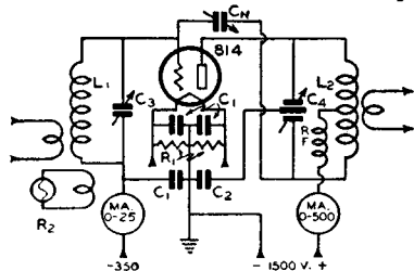
Wiring Diagram of the 100-Watt Grid-Modulated Stage
