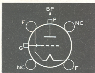
Tube Mounting Position VERTICAL—Base down only HORIZONTAL—Not recommended
