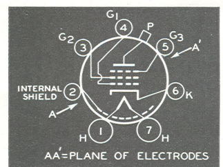
Tube Mounting Position VERTICAL or HORIZONTAL
