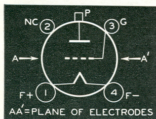
Bottom View of 809 and 1623 Socket Connections
