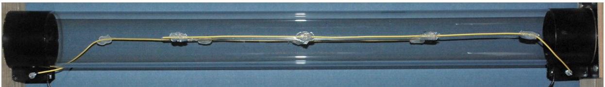
SSQ-BAT with side electrode wires permanently mounted in place using Silicone adhesive. This is just one way in which to attach the Side Wires to the plasma tube.
