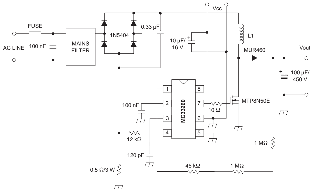
Figure 37. Compact Power Factor Correction
