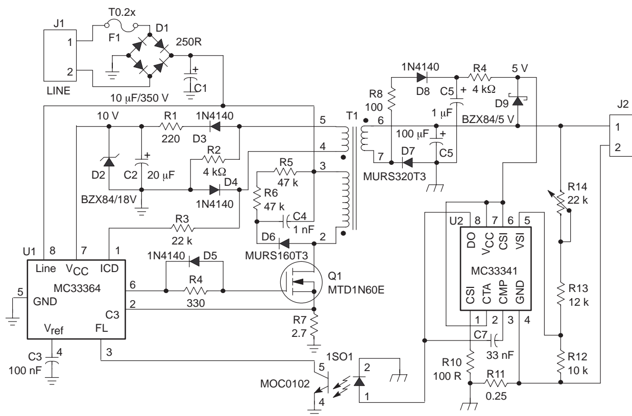
Figure 45. AC–DC Battery Charger – Constant Current with Voltage Limit
