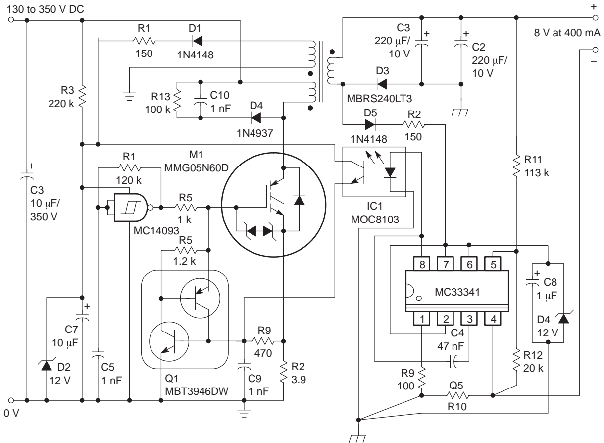
Figure 41. Low-Cost Offline IGBT Battery Charger
