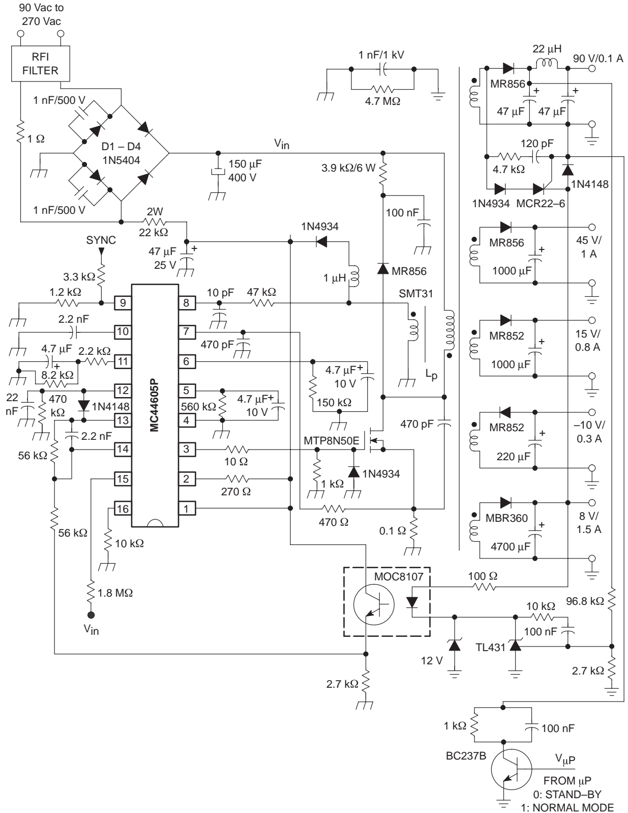
Figure 38. Monitor Pulsed-Mode SMPS
