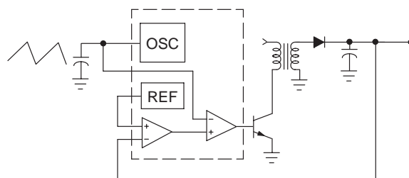
Figure 22. Voltage-Mode Control
