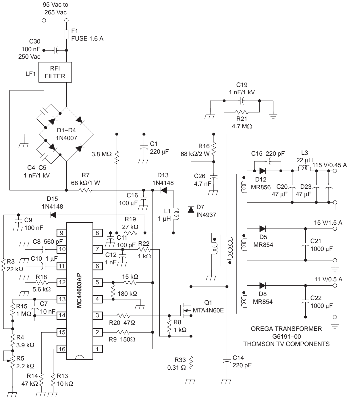
Figure 39. 70 W Wide Mains TV SMPS
