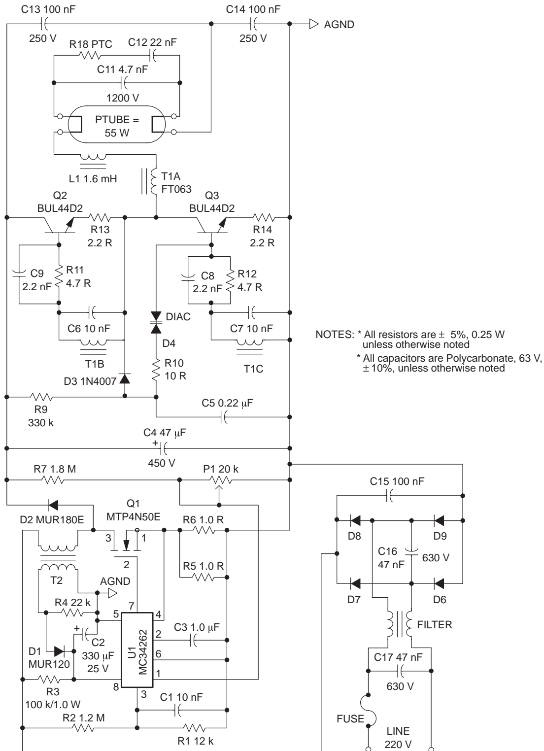
Figure 43. Efficient Safety Circuit for Electronic Ballast
