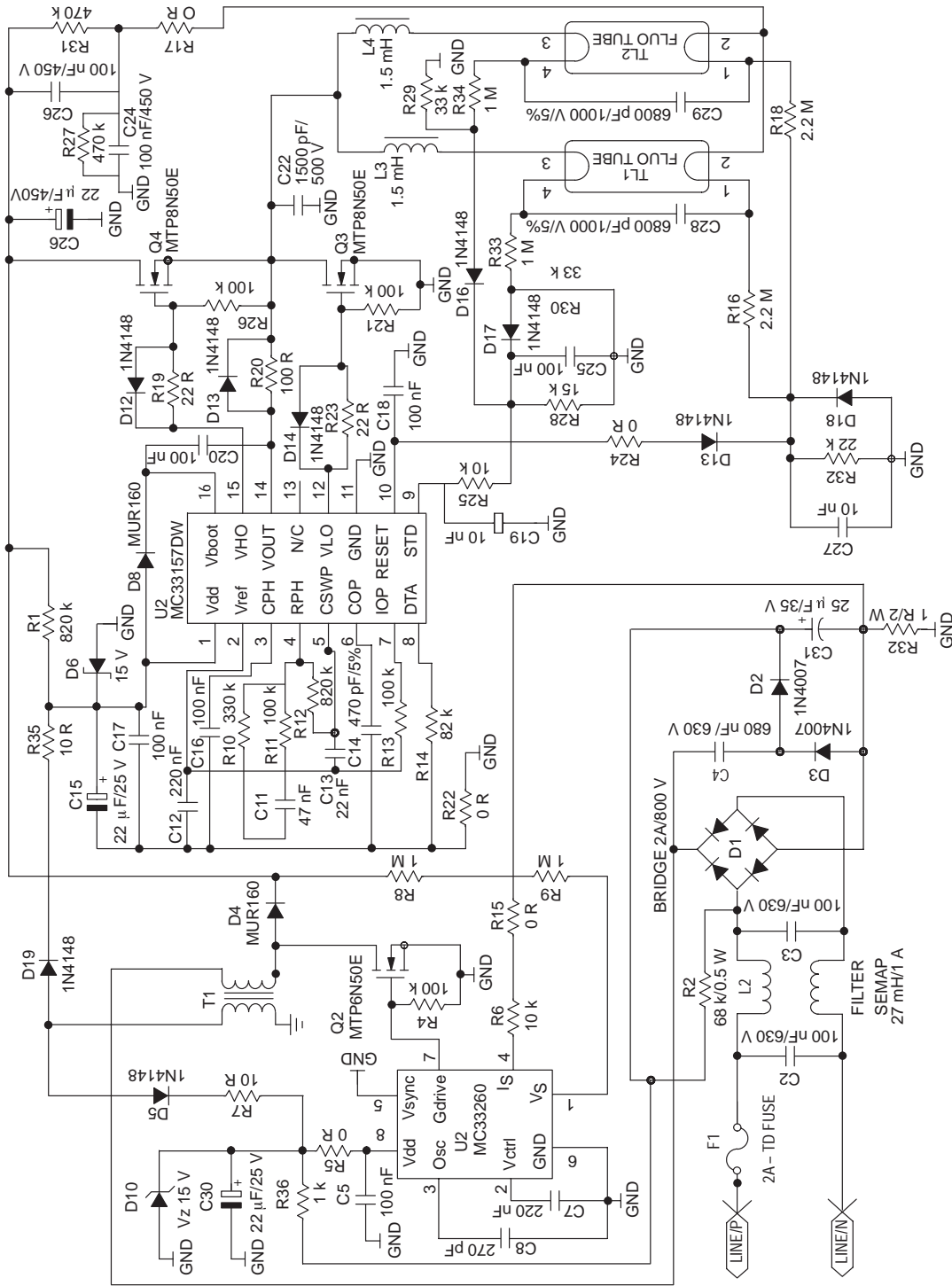
Figure 44. Lamp Ballast with Power Factor Correction (Evaluation Board)
