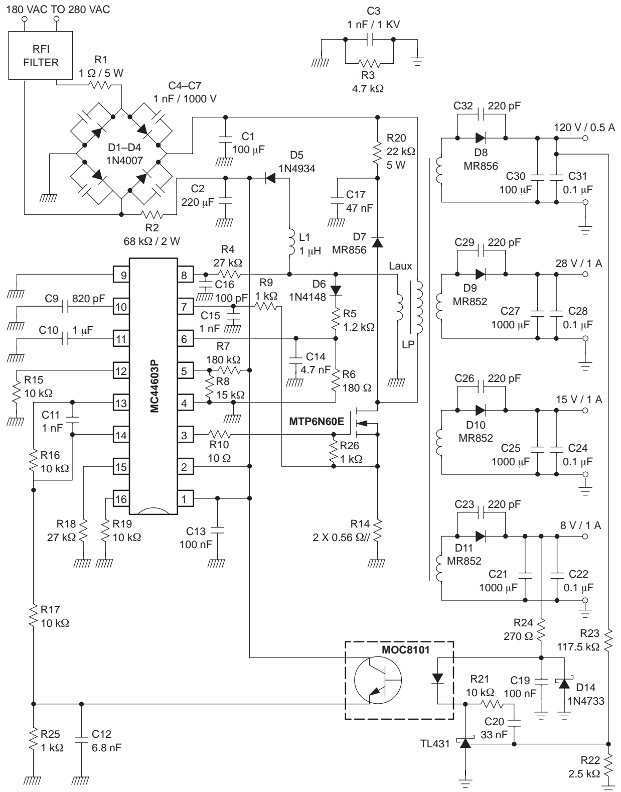
Figure 42. 110 W Output Flyback SMPS
