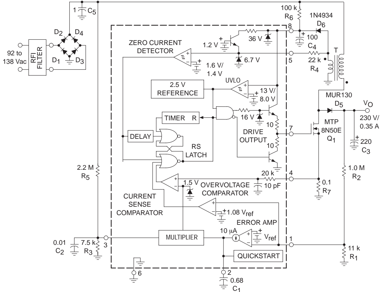
Figure 36. 80 W Power Factor Controller
