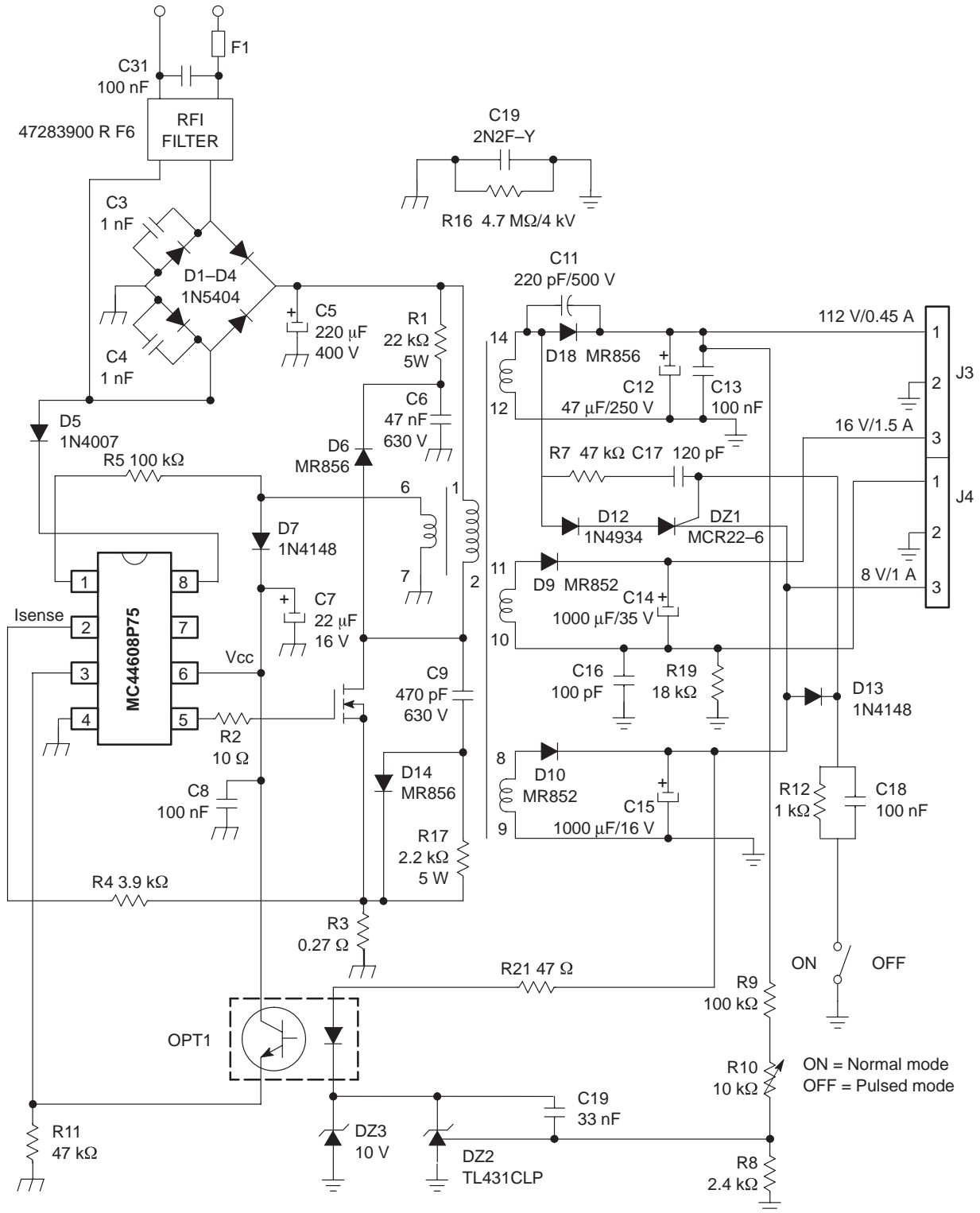
Figure 40. Wide Mains 100 W TV SMPS with Secondary Reconfiguration for 1.3 W TV Stand-by
