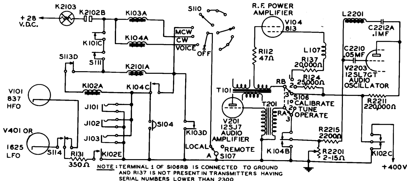
Figure 4-4. Emission Selection and Control Circuits
