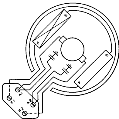
Figure 5-28. Emerson Type NY-818C-A Motor
