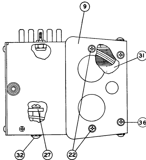
Figure 5-19. 410 0008 00 Keying Relay (K102)
