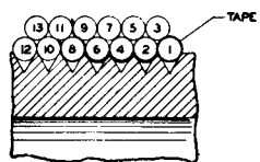
FIGURE 1 METHOD OF TAPING START OF WINDING AND SEQUENCE OF DOUBLE BANK WINDING
