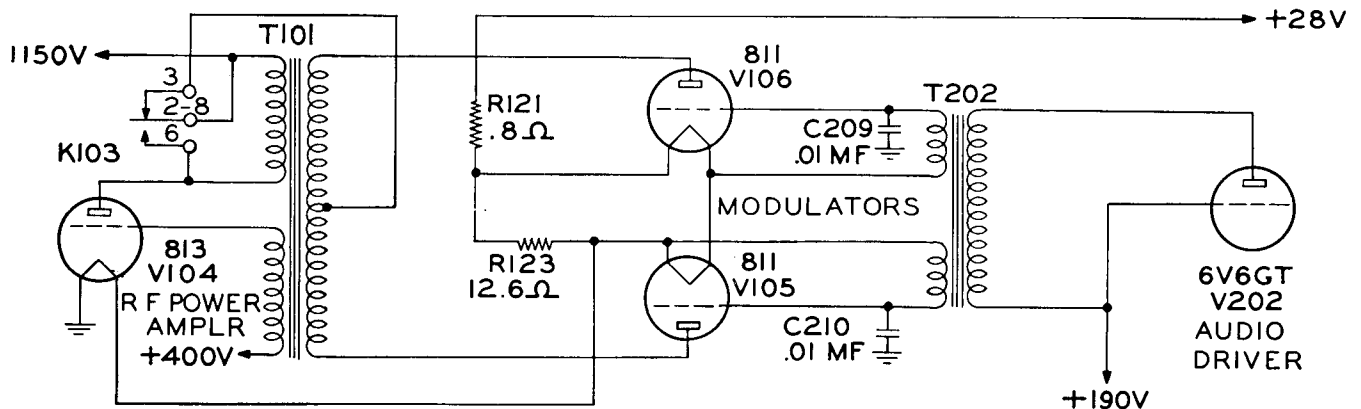
Figure 4-7. Modulator Circuit
