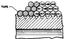
FIGURE 2 METHOD OF TAPING END OF WINDING AND SEQUENCE OF TRIPLE BANK WINDING
