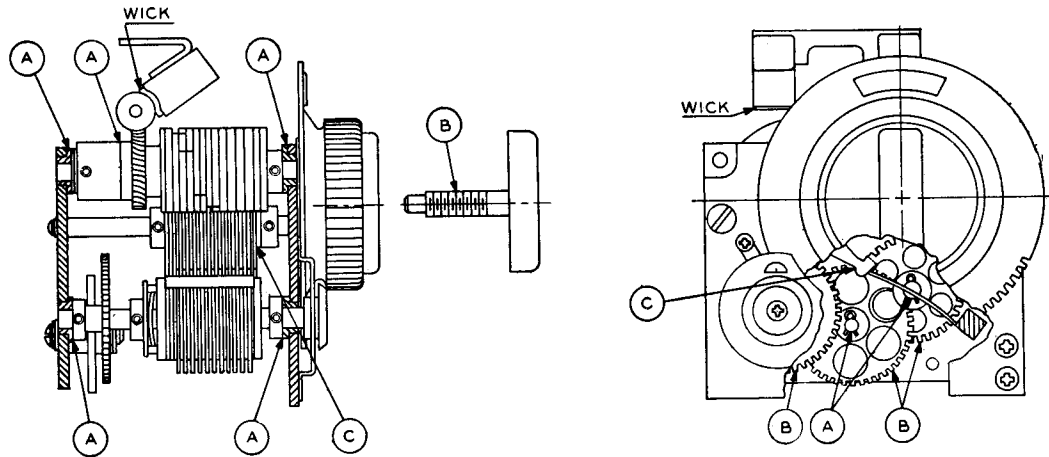
MULTITURN UNIT
