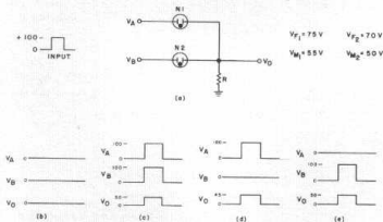
Fig. 3.10. Waveforms for Basic 2-Input "OR" Gate.
