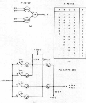
Fig. 3.14. Glow Lamp Logic Circuit (Direct-Coupled).
